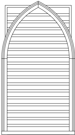
24"x48" Gothic Top with Square Jamb
